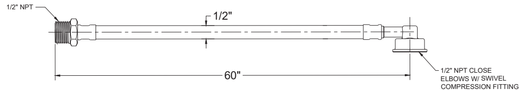
60" BRAIDED WATER SUPPLY LINE 1X PIECE PER KIT
