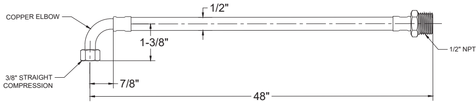
48" BRAIDED WATER SUPPLY LINE WITH 90° COPPER ELBOW 2X PIECES PER KIT
