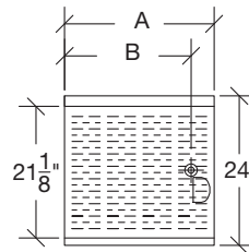
KR24 Standard Drainboard
