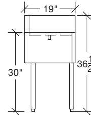
KR19 Corner Drainboard with Left Return
