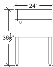
KR24 Corner Drainboard with Left Return
