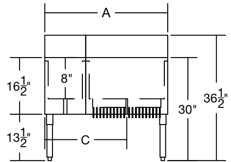
Front View - Cold plate models
