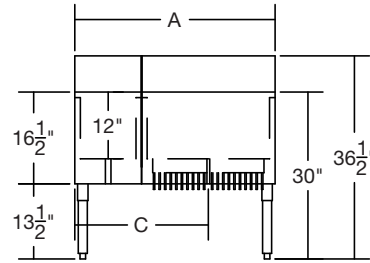
Front View - Cold plate models
