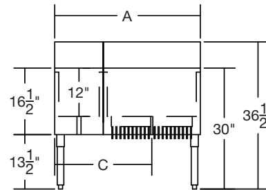
Front View - Cold plate models
