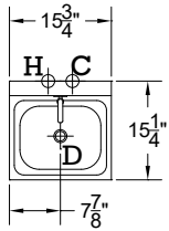
HS-15 Weight: 19 lbs.
