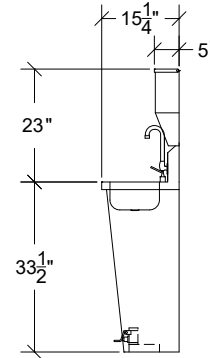
HS-39 Weight: 38 lbs.
