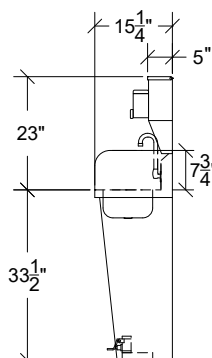
HS-42 Weight: 42 lbs.
