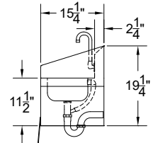
HS-40 Weight: 34 lbs.
