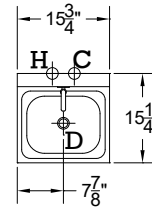
HS-16 Weight: 27 lbs.
