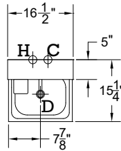
HS-16 Weight: 27 lbs.
