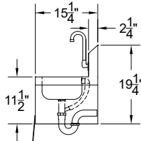
HS-14 Weight: 31 lbs.
