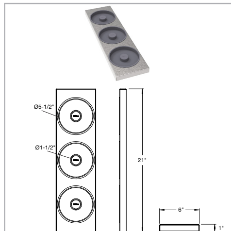
MW-MR6 - MoveWell Margarita Rimmer
