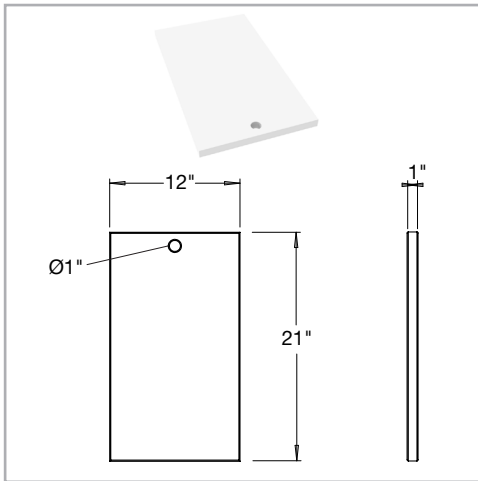
MW-CB12 - MoveWell Cutting Board, 12"W
