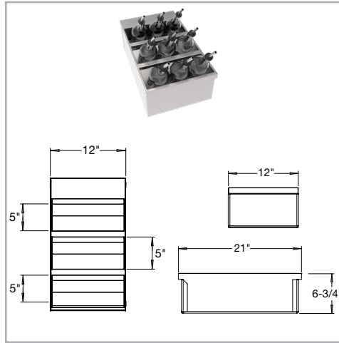
MW-SR12 - MoveWell Bottle 3-Tier Speed Rack, 12"W
