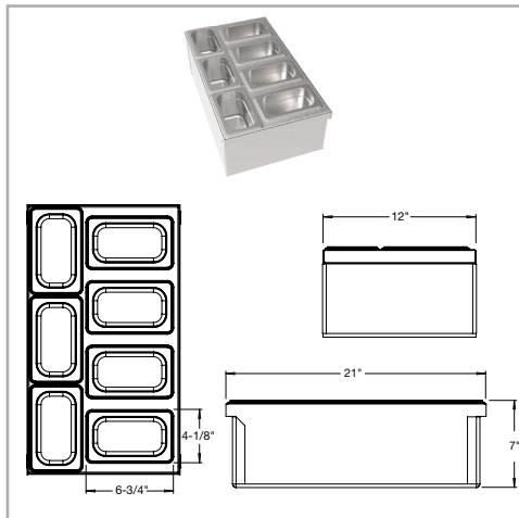
MW-CT12 - MoveWell Condiment Tray, 12"W
