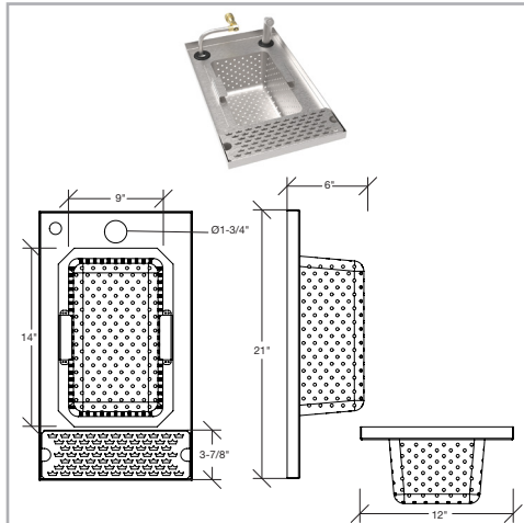
MW-WD12 - MoveWell Wash Down Dump Sink
