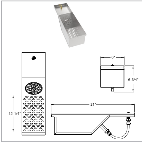
MW-SJ6 - MoveWell Spray Jet Dump Sink 6"W
