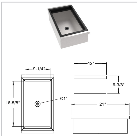
MW-IB12 - MoveWell Insulated Ice Bin
