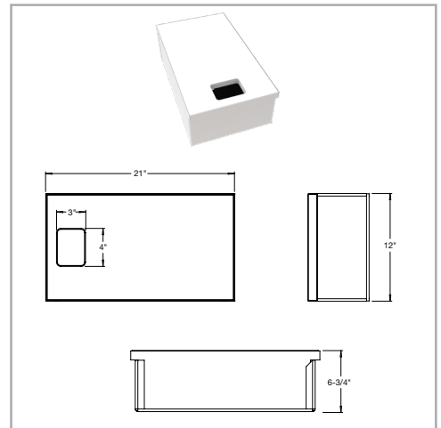
MW-CS12 - MoveWell Cutting Board with Trash Station
