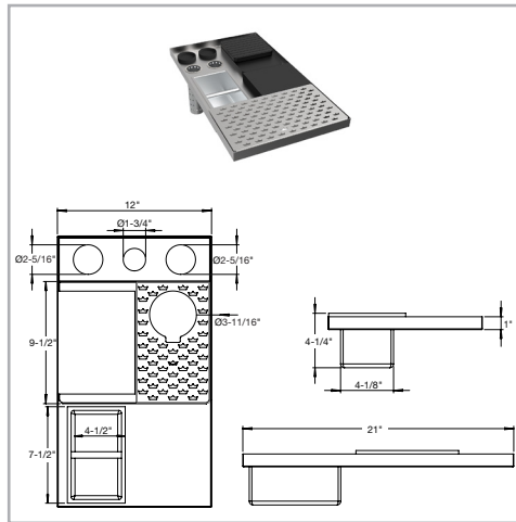
MW-CF12 - MoveWell Coffee Insert
