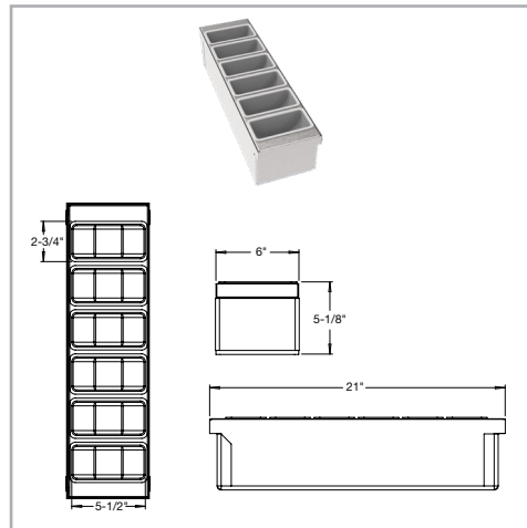
MW-CT6 - MoveWell Condiment Tray, 6"W
