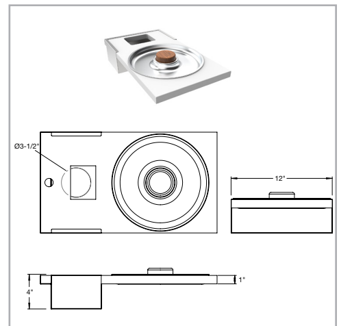
MW-OS12 - MoveWell Oyster Insert
