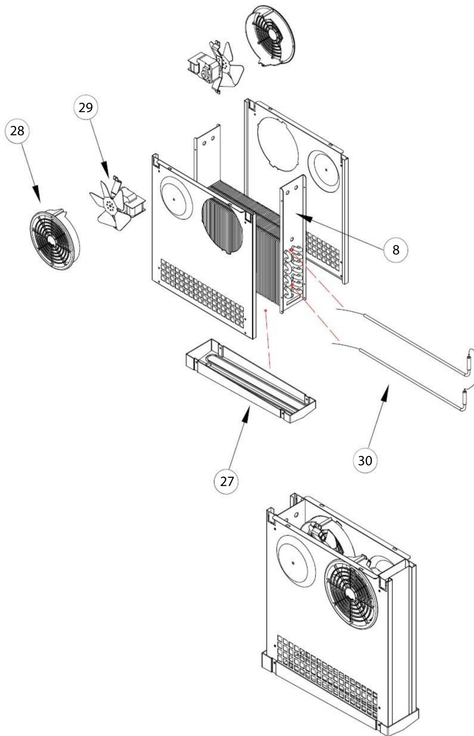
Undercounter - Evap Coil Group Detail
